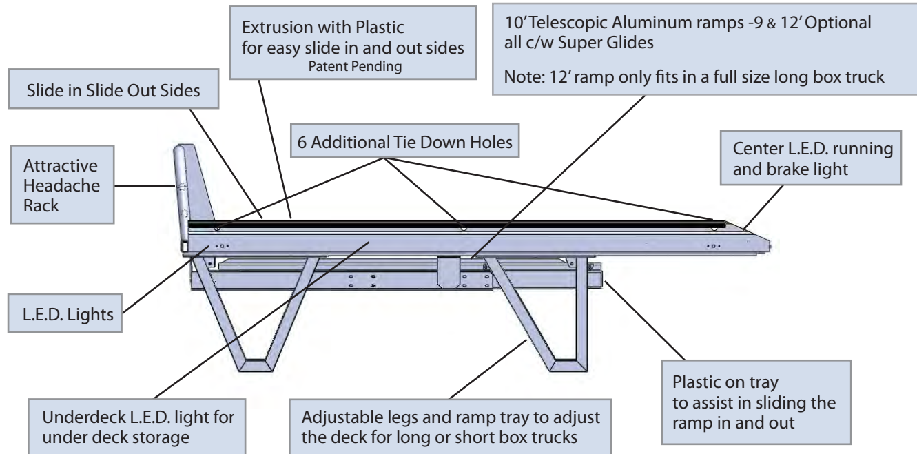
Ramp Tray
